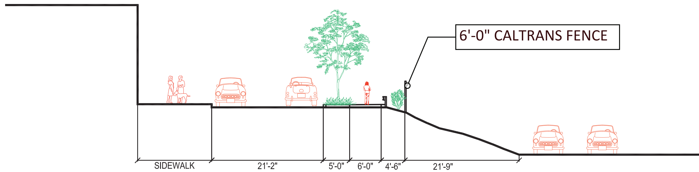
SECTION C-C
