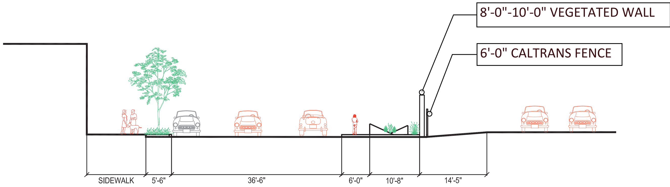
SECTION B-B
