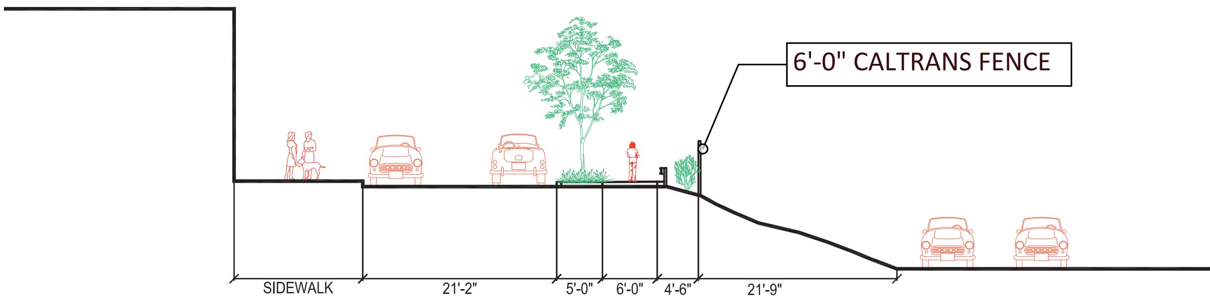
SECTION C-C
